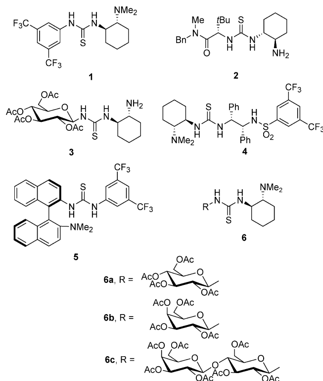
Figure 1. Thiourea organocatalysts.
